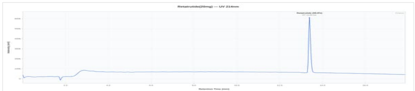
RT20 20mg - CP01260707220L: UV Chromatogram
